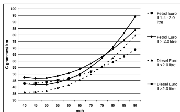
Figure 1: Changes in CO 2 emissions with speed Source: NETCEN National Atmospheric Emissions Inventory
